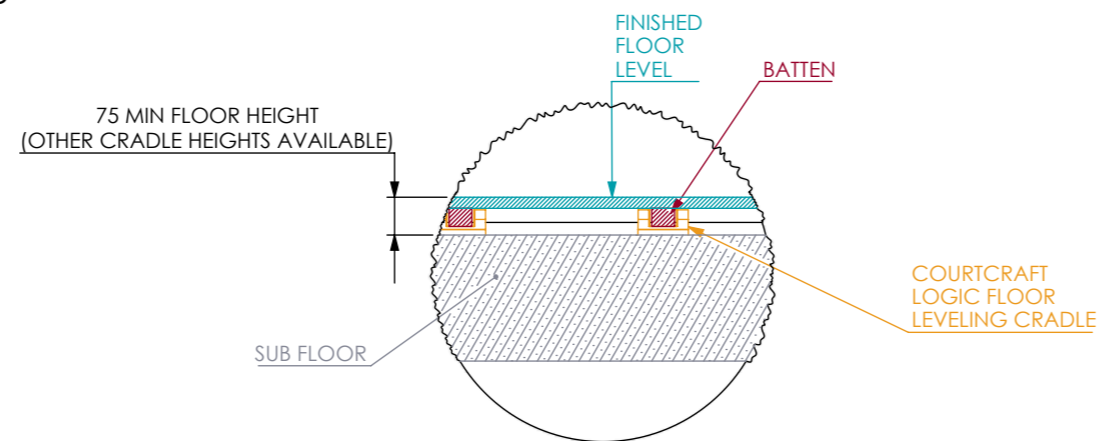
DETAIL B LOGIC FLOOR SYSTEM SCALE 1 : 15
